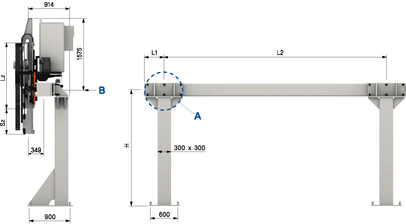
View B
