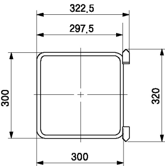
View X
